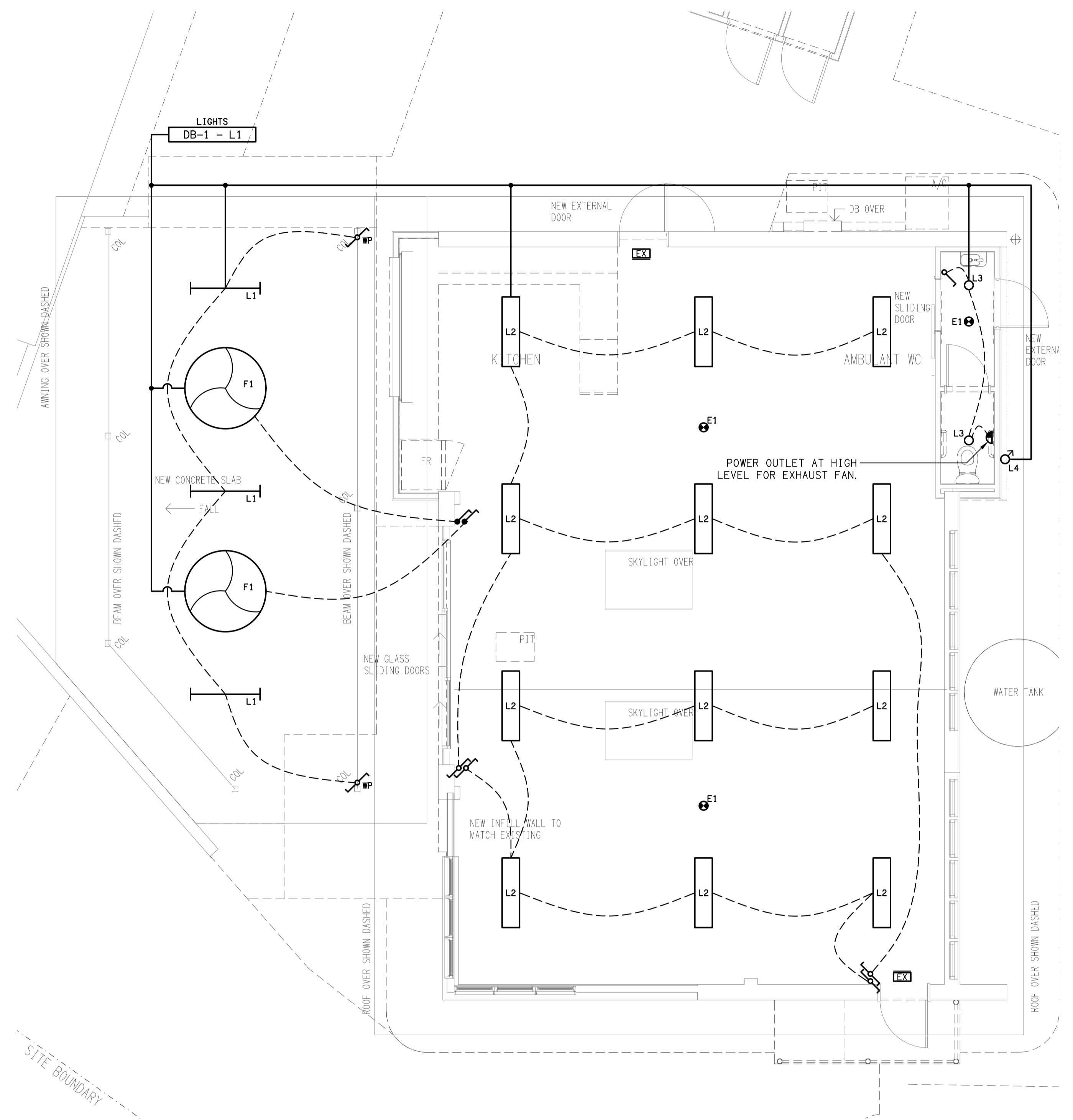
BUILDING 1 REFLECTED CEILING PLAN SCALE 1:50
